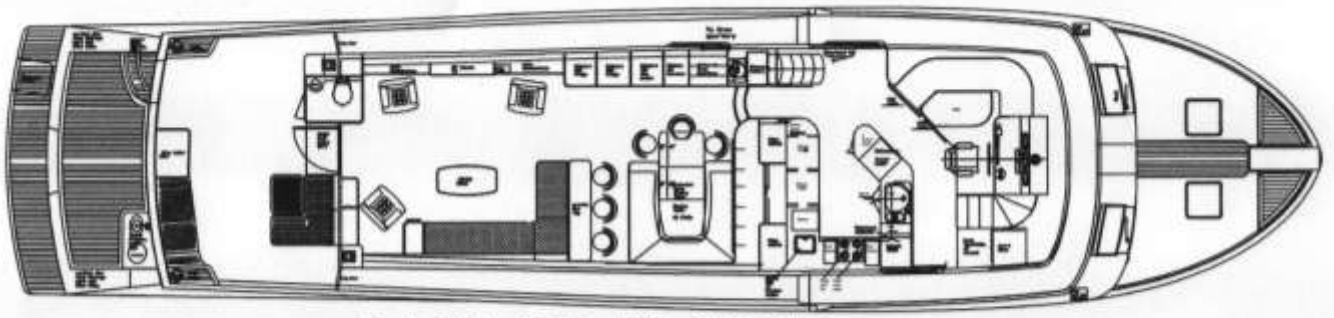
Marlow Explorer 86 Cockpit Motor Yacht Interior Arrangement
