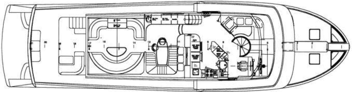
Marlow Explorer 72C & 78E Standard Interior Arrangement
