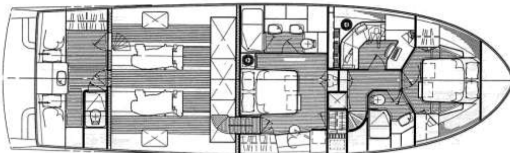
Marlow Explorer 61E Euro Interior Arrangement
