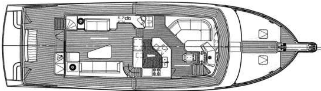
Marlow Explorer 61E Euro Interior Arrangement
