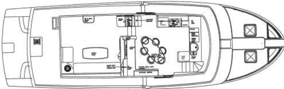
Marlow Explorer 57E Command Bridge Alternate Arrangement
